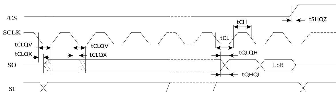
Figure 47. Output Timing
